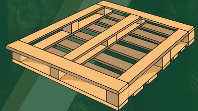
Perimeter Base
